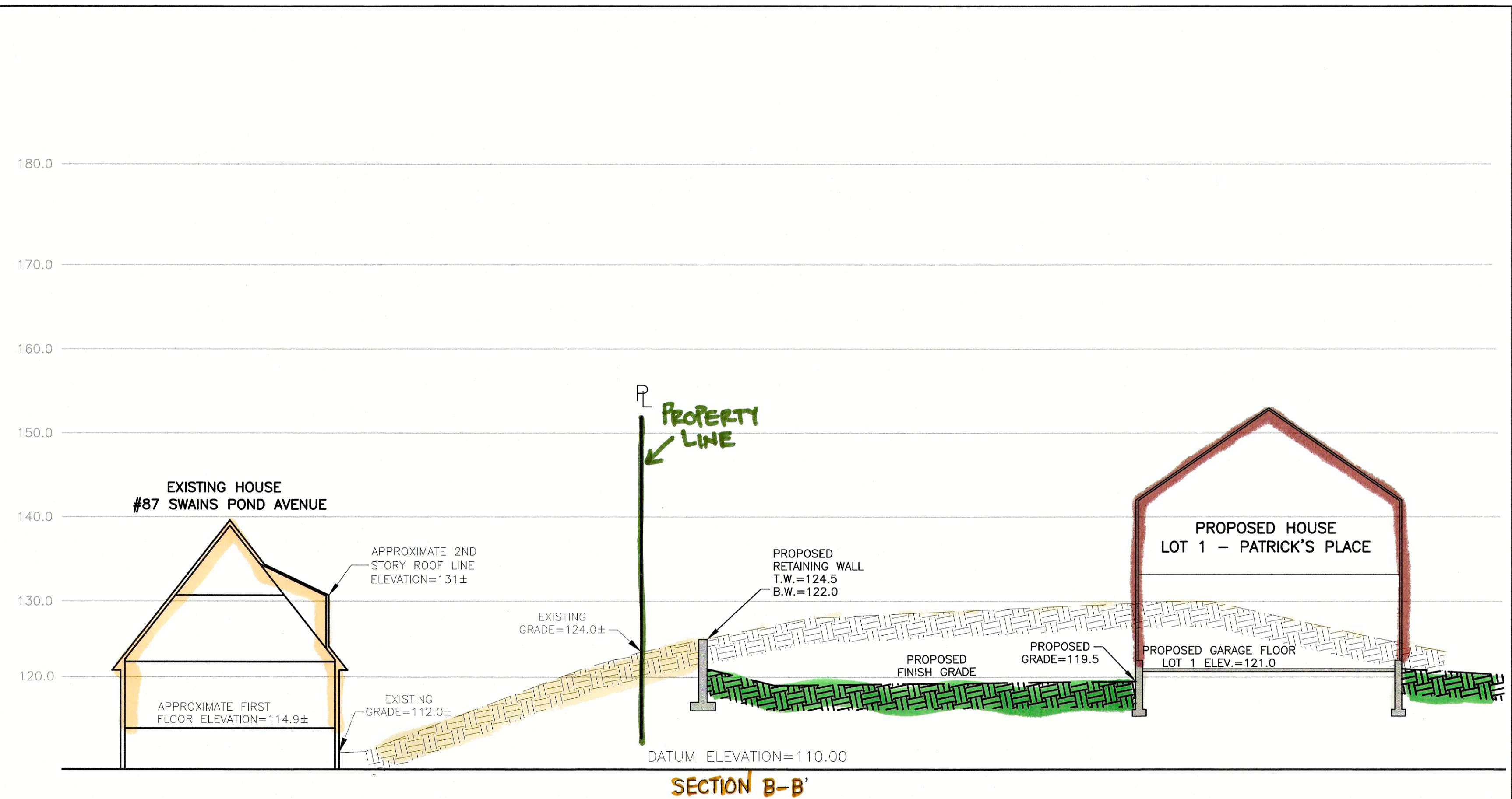
PROFILE VIEW 1"=10' VERTICAL 1"=10' HORIZONTAL
